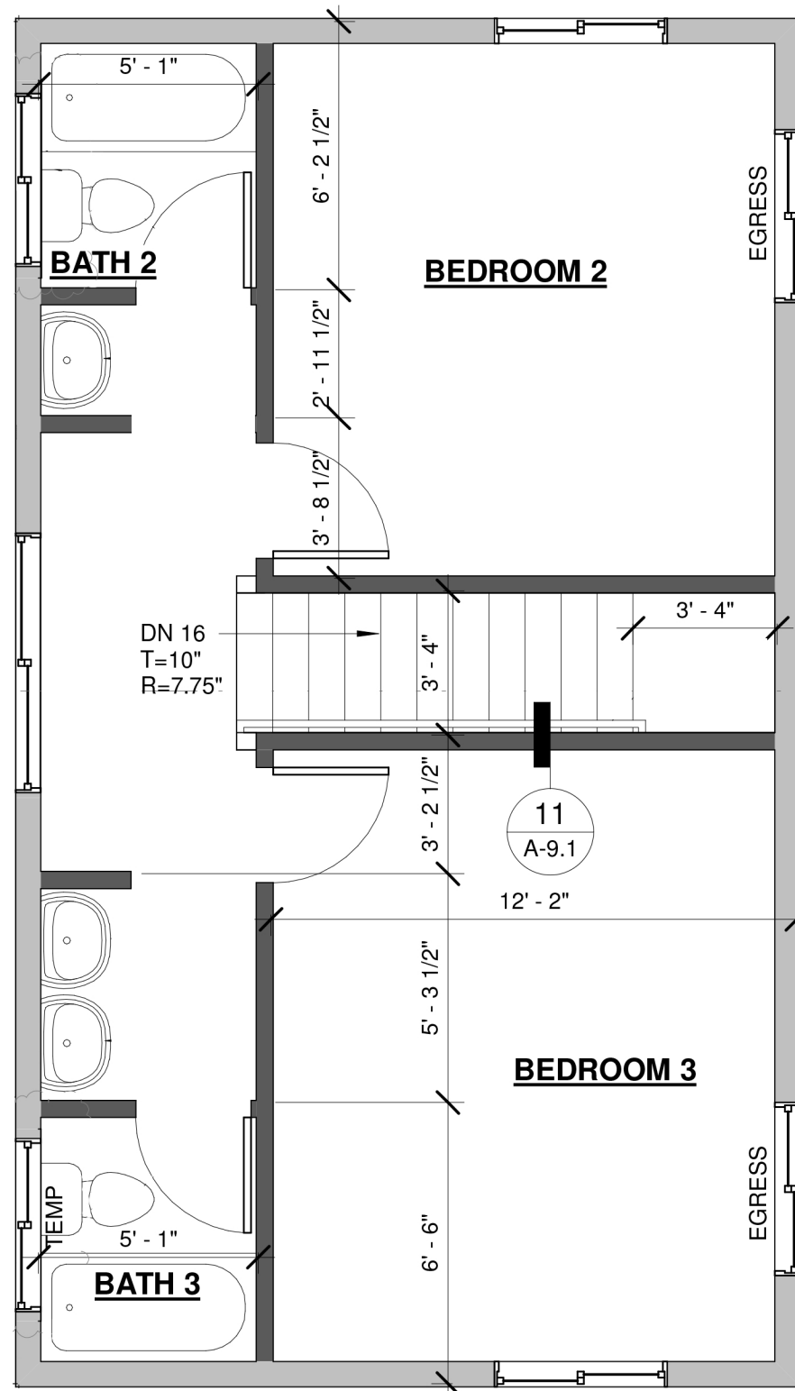
2ND FLOOR 567 SQUARE FEET
