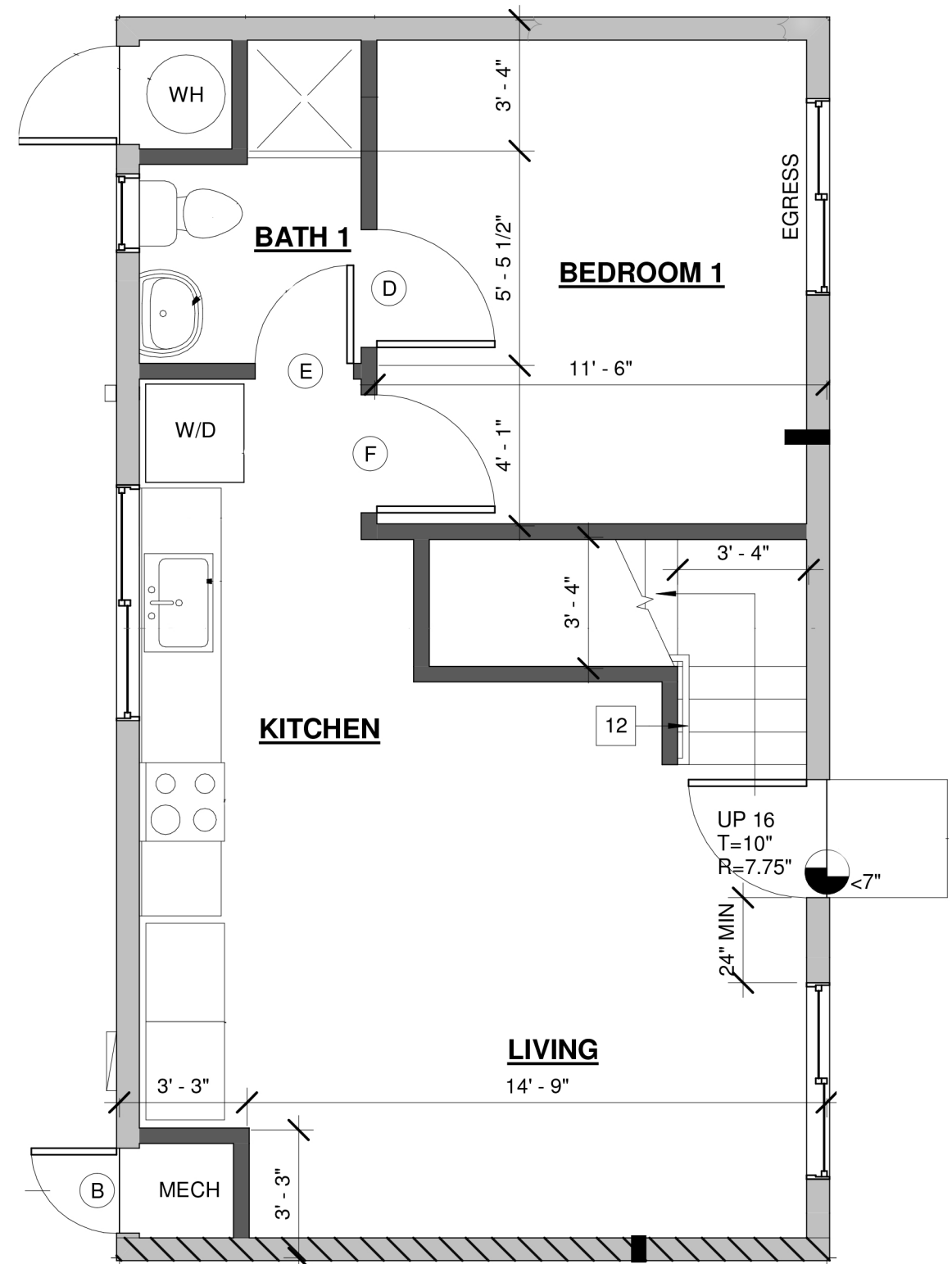
1ST FLOOR 567 SQUARE FEET
